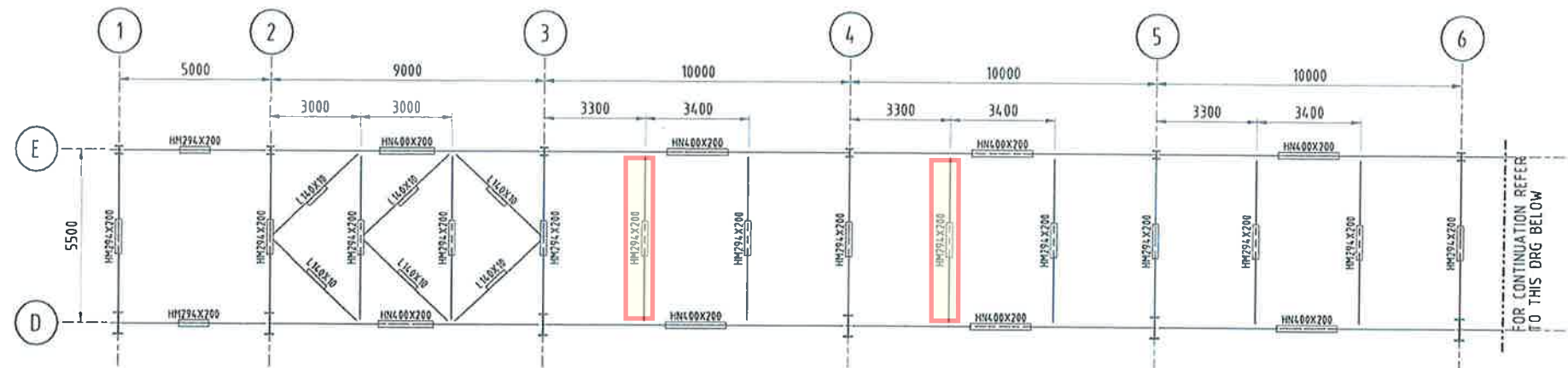
PART PLAN AT EL 8.900m TOS ALL DIAGONAL HORIZONTAL BRACING TO BE (-0.125m) U.N.O
